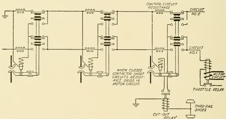
Fig. 66. Diagram of Interlocks, Sprague-General Electric Automatic Control
